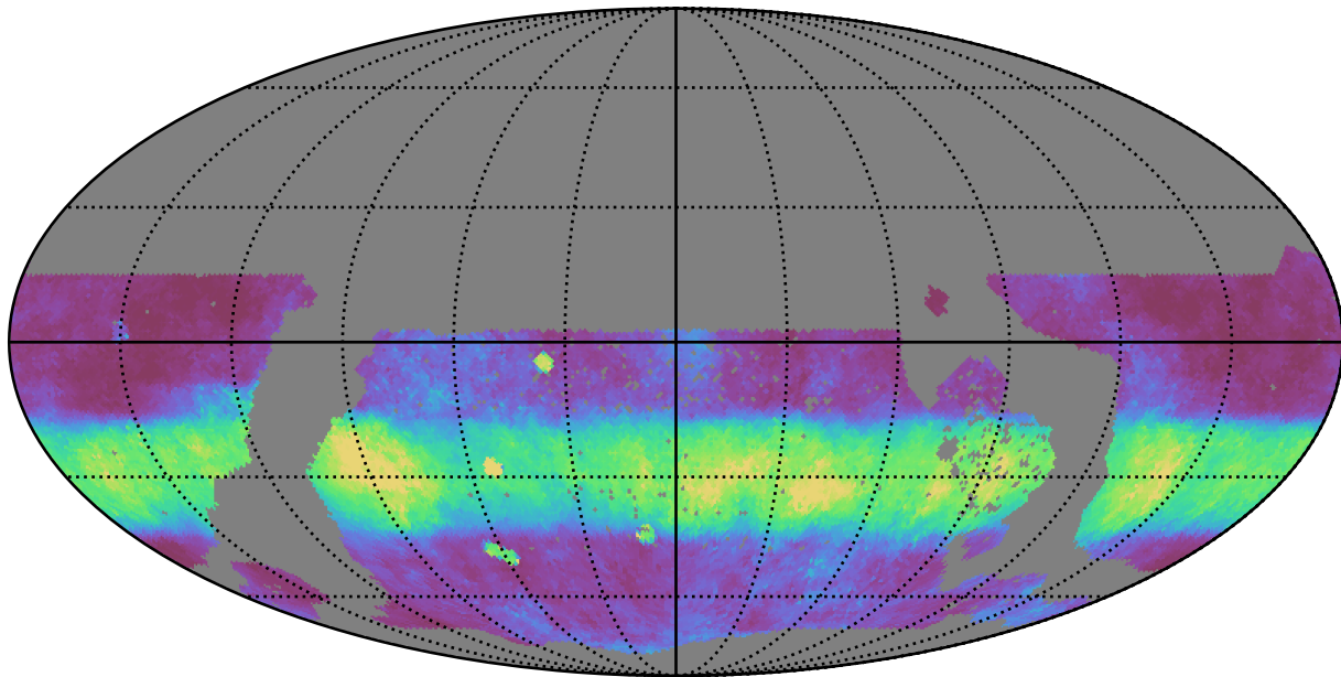
too_5_4v3.4_10yrs WFD i band: Median normairmass
