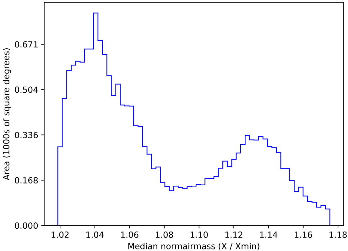
too_5_4v3.4_10yrs WFD i band: Median normairmass
