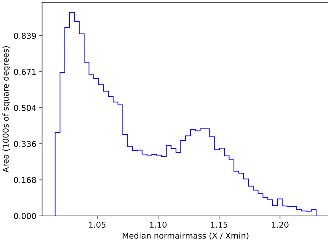
too_5_4v3.4_10yrs WFD g band: Median normairmass
