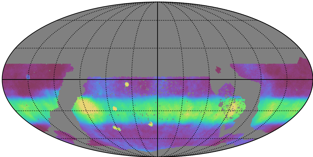
too_5_4v3.4_10yrs WFD all bands: Median normairmass
