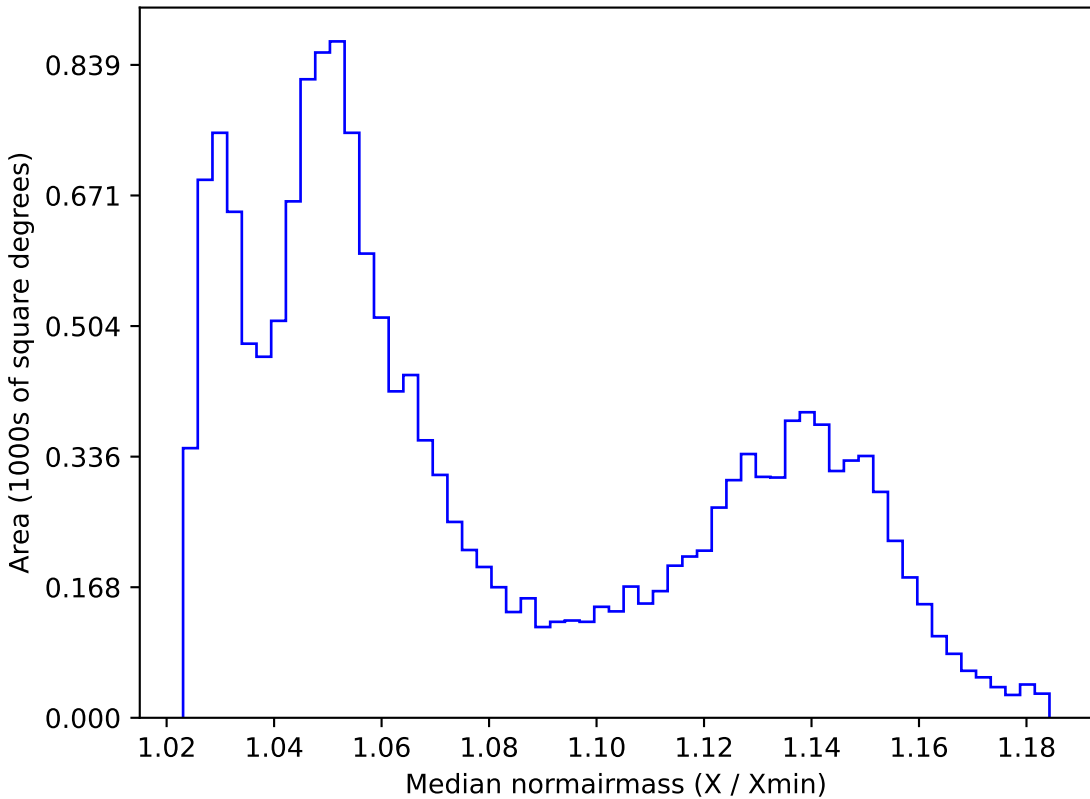
too_5_4v3.4_10yrs WFD all bands: Median normairmass
