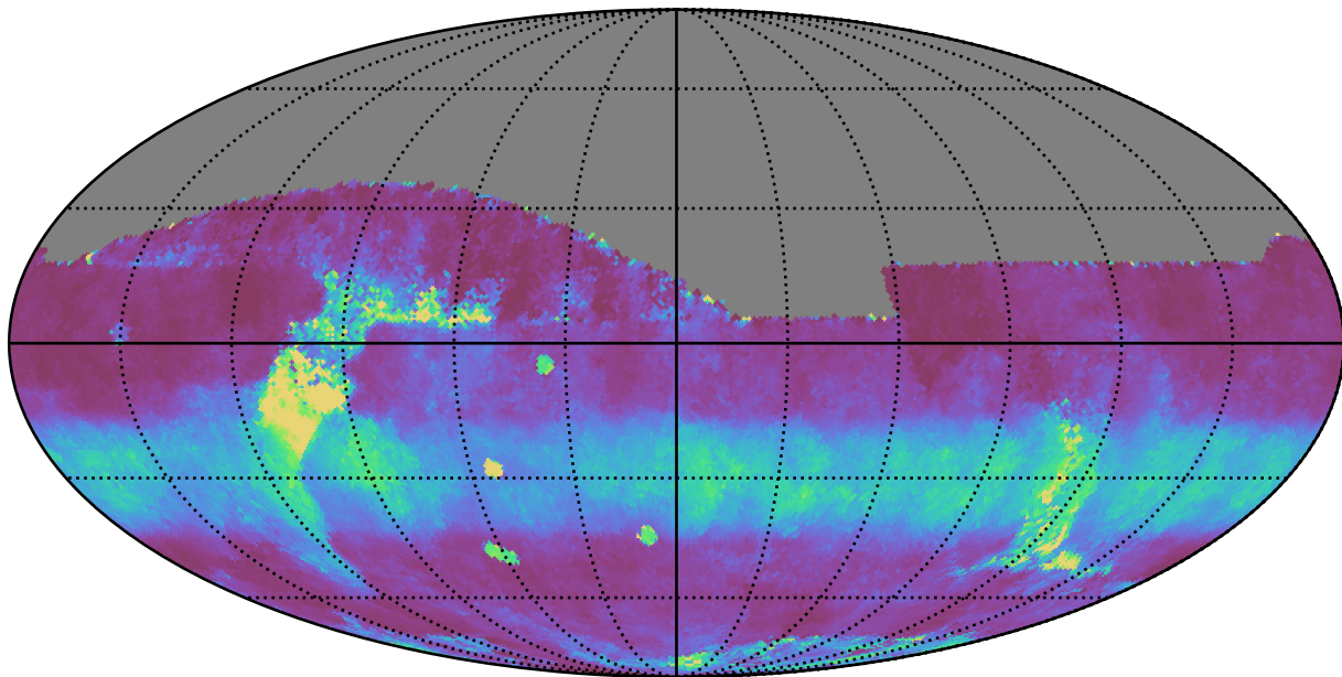
too_5_4v3.4_10yrs All sky z band: Median normairmass
