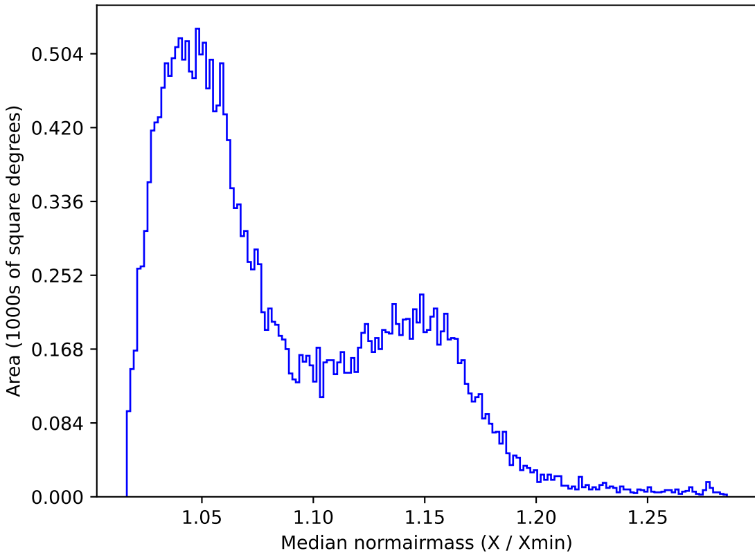
too_5_4v3.4_10yrs All sky z band: Median normairmass
