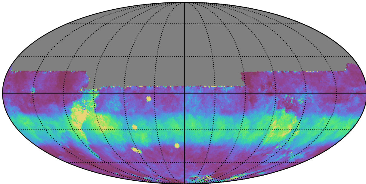
too_5_4v3.4_10yrs All sky y band: Median normairmass
