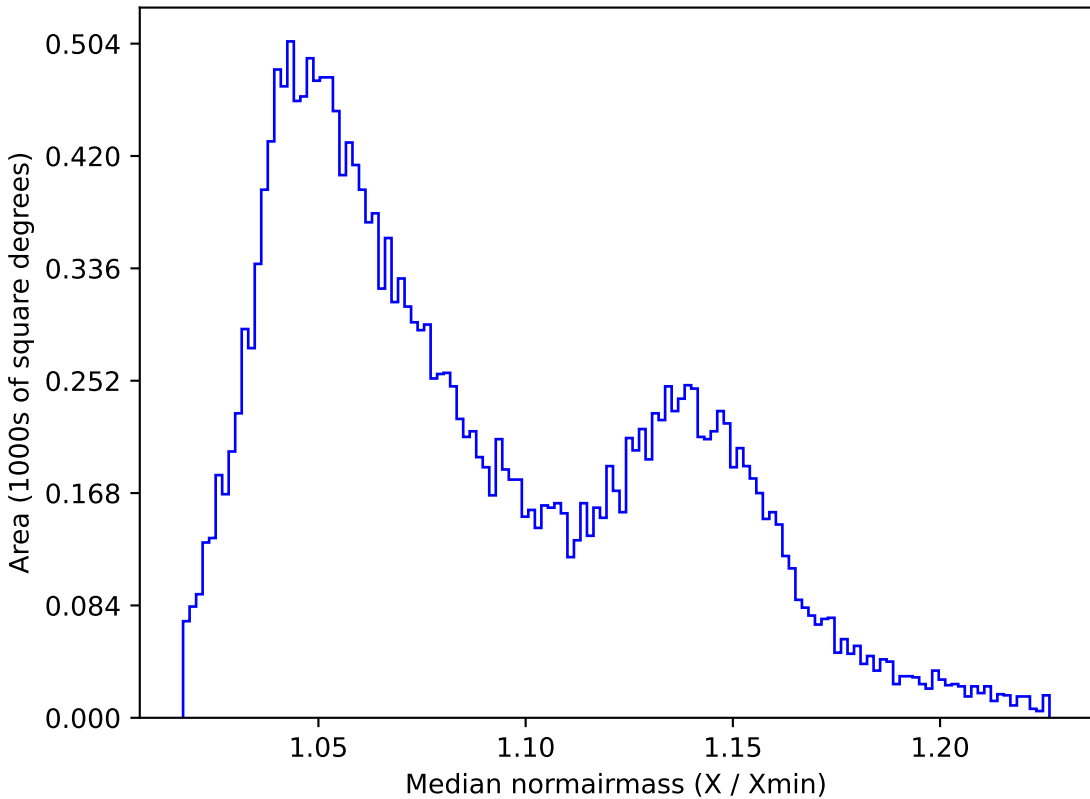
too_5_4v3.4_10yrs All sky y band: Median normairmass
