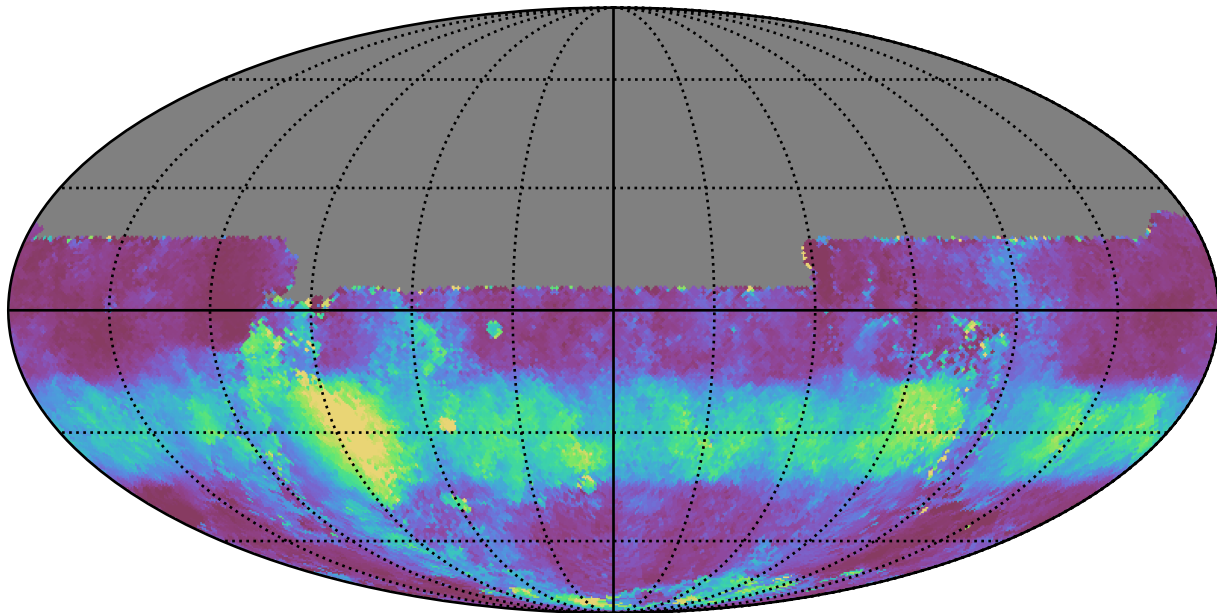
too_5_4v3.4_10yrs All sky u band: Median normairmass
