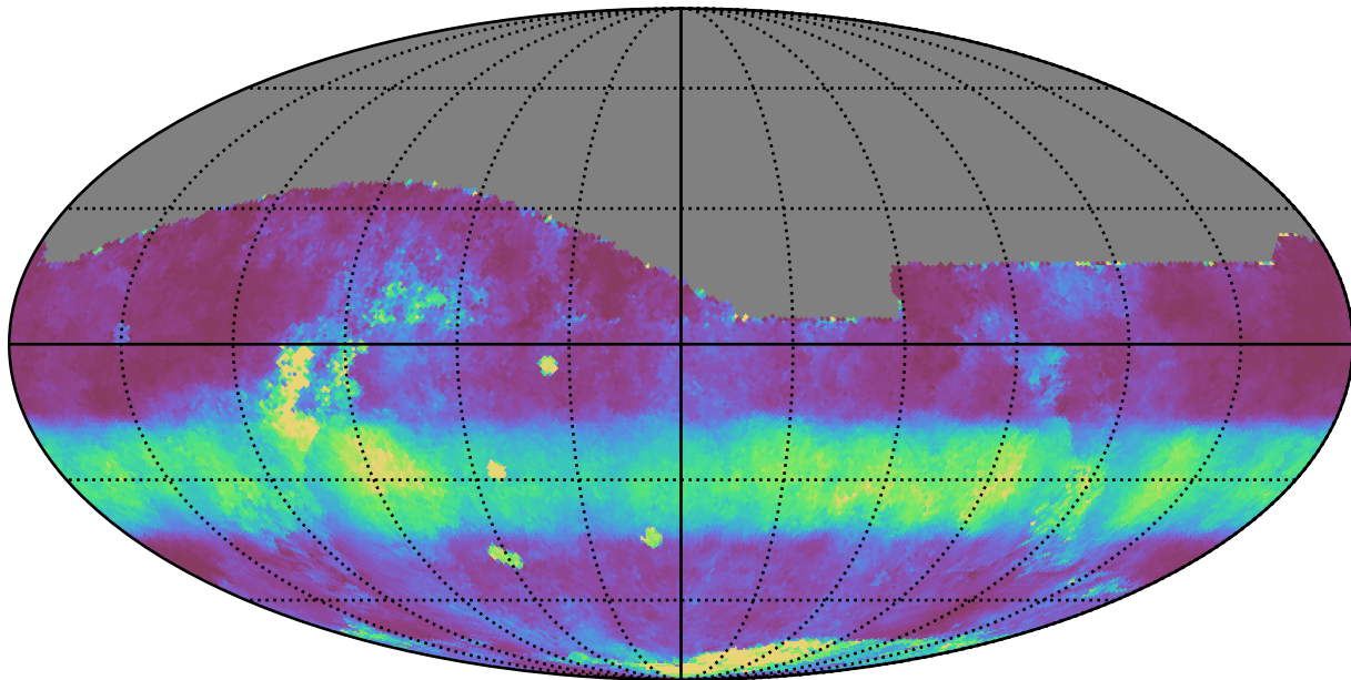
too_5_4v3.4_10yrs All sky r band: Median normairmass
