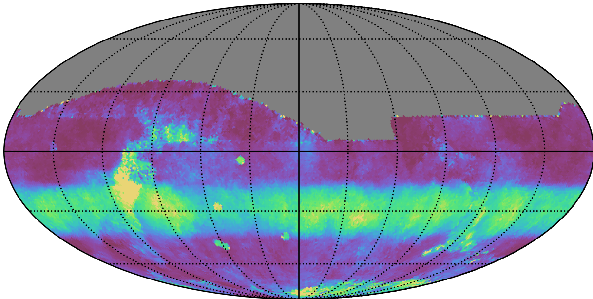
too_5_4v3.4_10yrs All sky i band: Median normairmass
