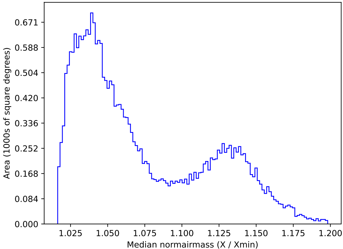
too_5_4v3.4_10yrs All sky i band: Median normairmass
