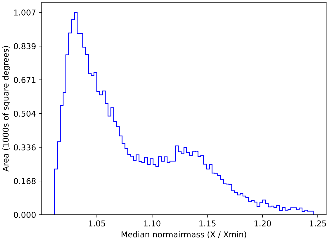
too_5_4v3.4_10yrs All sky g band: Median normairmass
