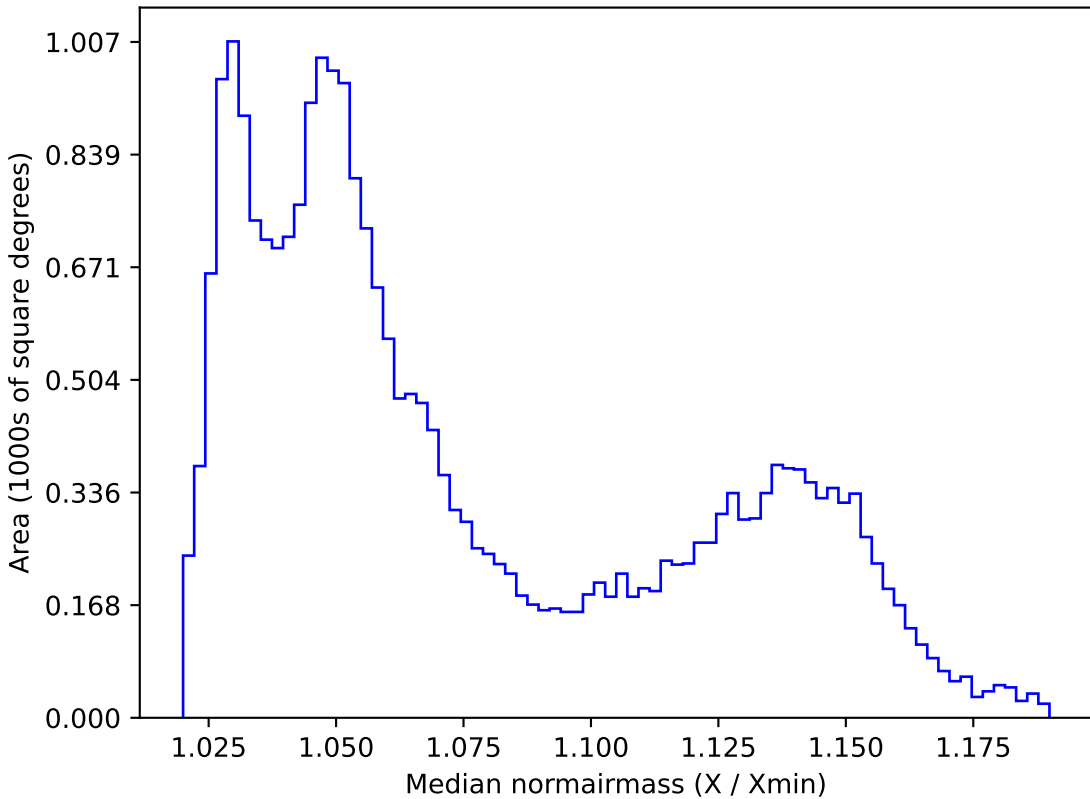
too_5_4v3.4_10yrs All sky all bands: Median normairmass
