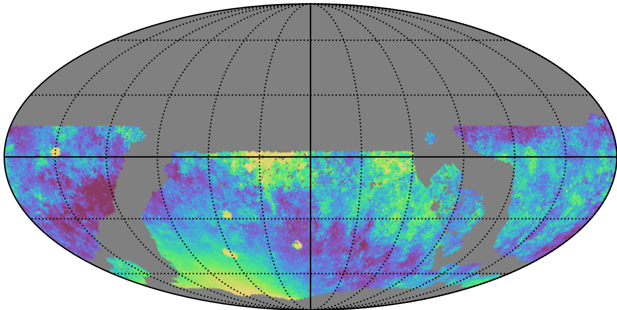
too_5_4v3.4_10yrs WFD z band: Median moonDistance
