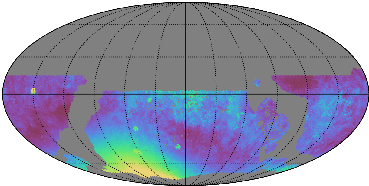
too_5_4v3.4_10yrs WFD y band: Median moonDistance
