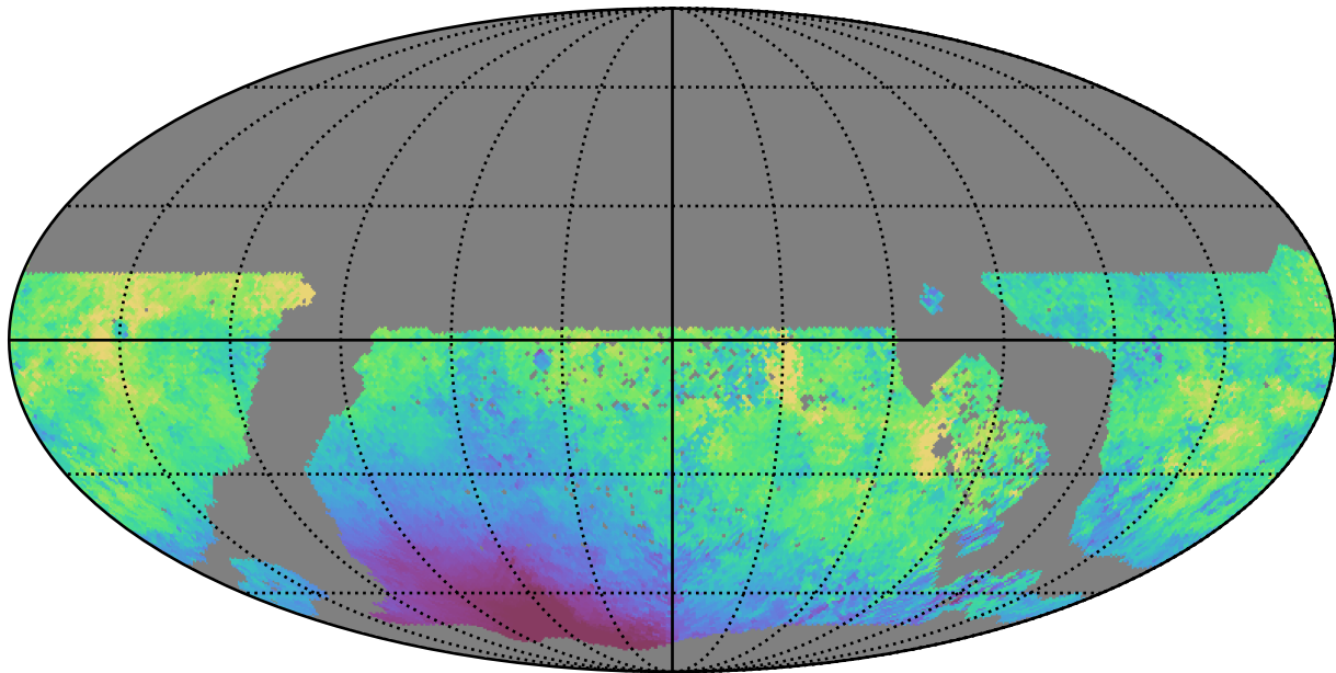
too_5_4v3.4_10yrs WFD u band: Median moonDistance
