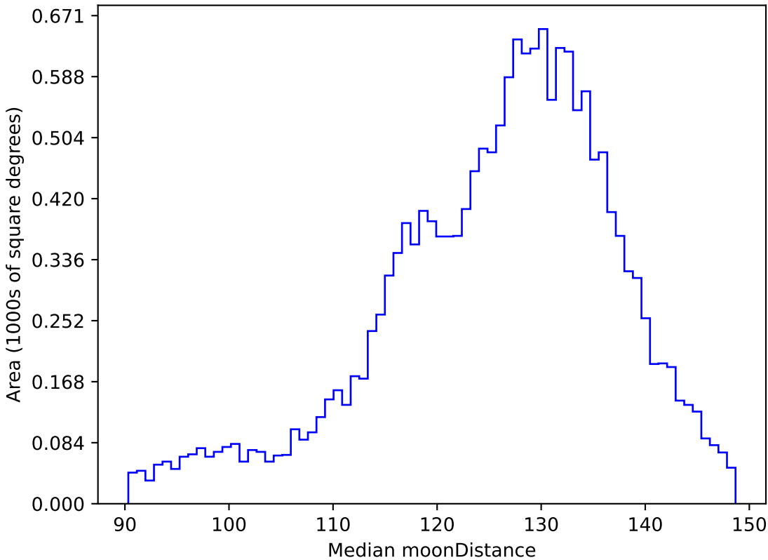
too_5_4v3.4_10yrs WFD u band: Median moonDistance
