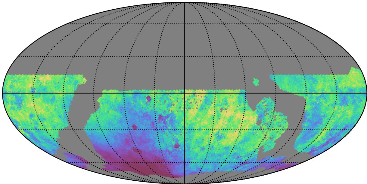
too_5_4v3.4_10yrs WFD r band: Median moonDistance
