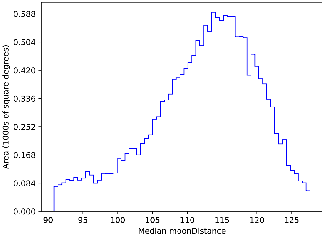
too_5_4v3.4_10yrs WFD r band: Median moonDistance
