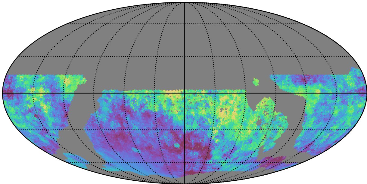
too_5_4v3.4_10yrs WFD i band: Median moonDistance
