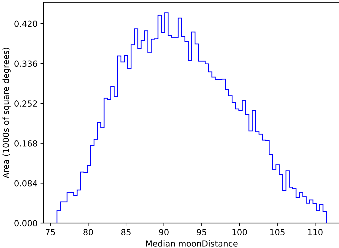
too_5_4v3.4_10yrs WFD i band: Median moonDistance
