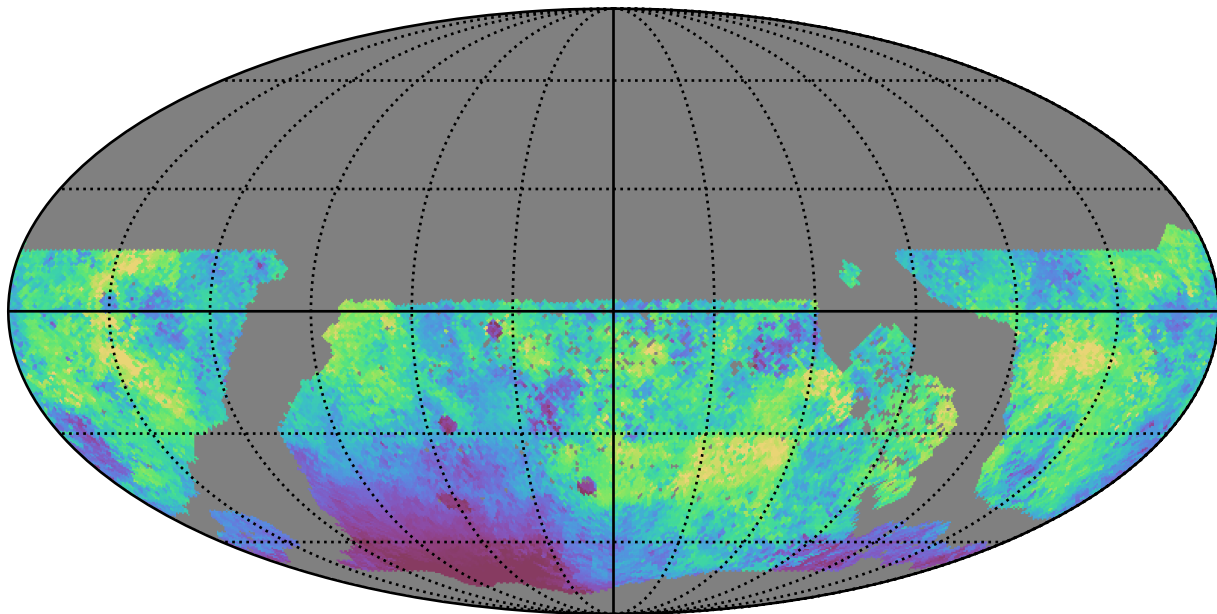
too_5_4v3.4_10yrs WFD g band: Median moonDistance
