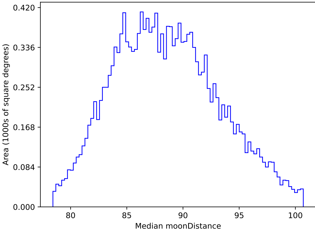
too_5_4v3.4_10yrs WFD all bands: Median moonDistance
