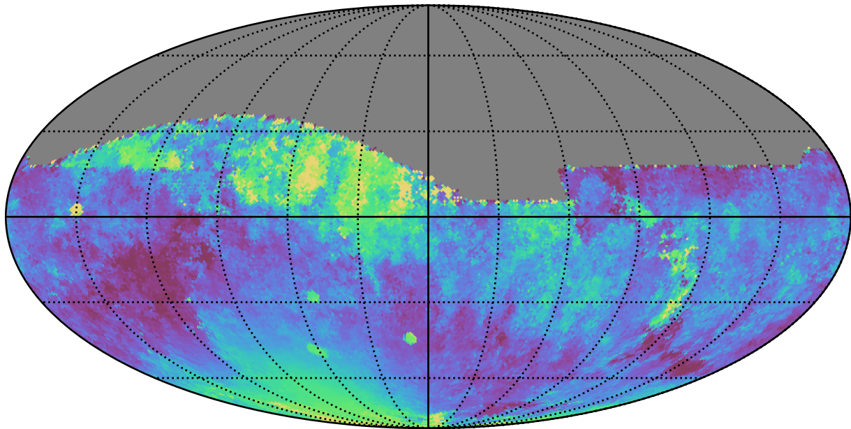
too_5_4v3.4_10yrs All sky z band: Median moonDistance
