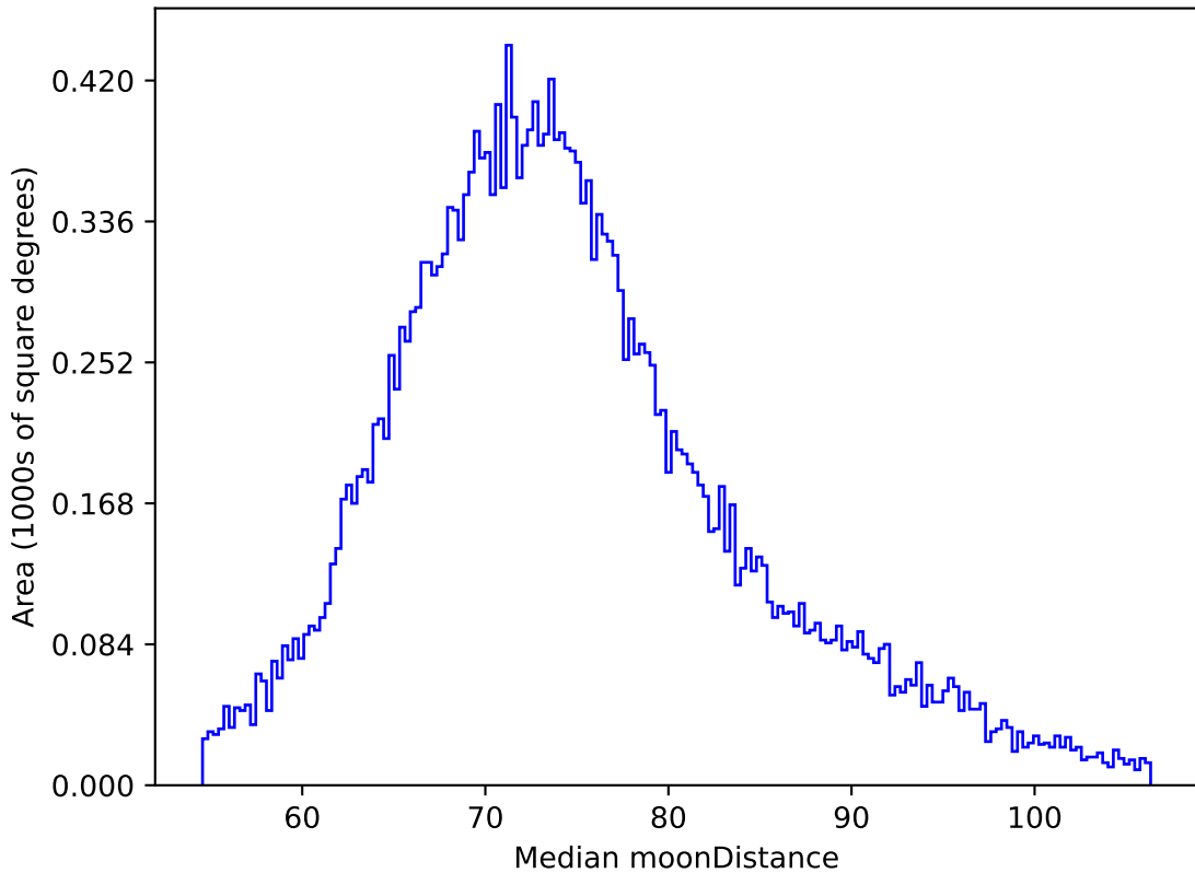
too_5_4v3.4_10yrs All sky z band: Median moonDistance
