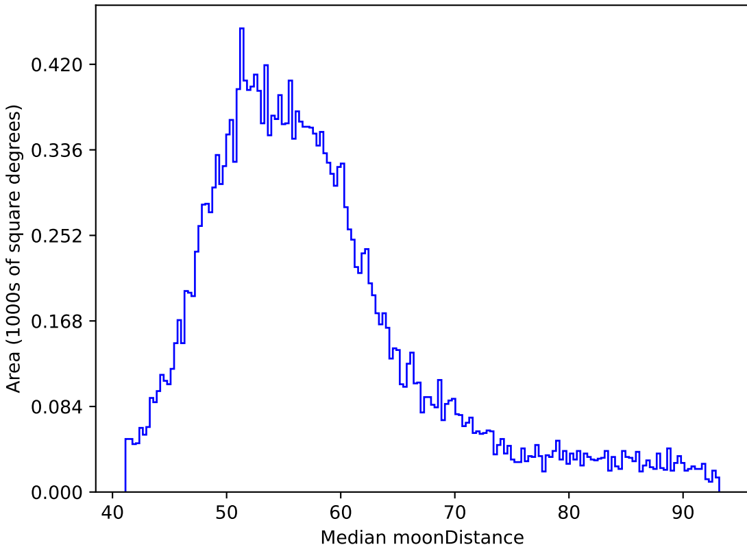
too_5_4v3.4_10yrs All sky y band: Median moonDistance
