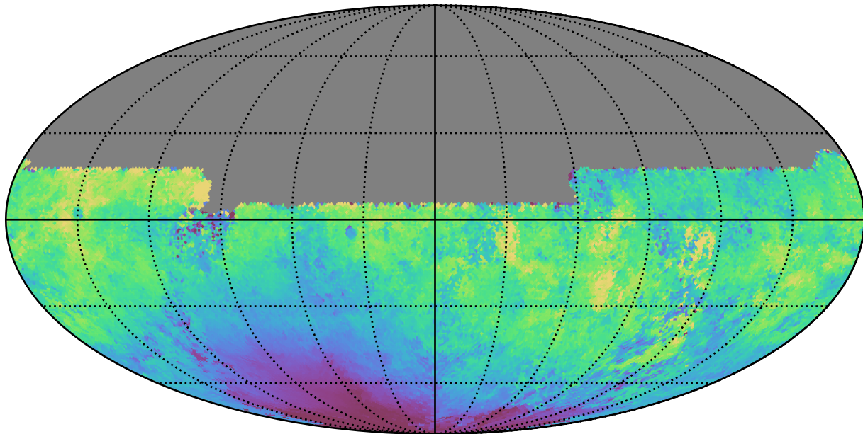
too_5_4v3.4_10yrs All sky u band: Median moonDistance
