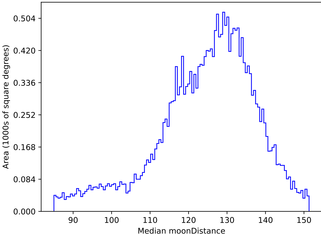
too_5_4v3.4_10yrs All sky u band: Median moonDistance
