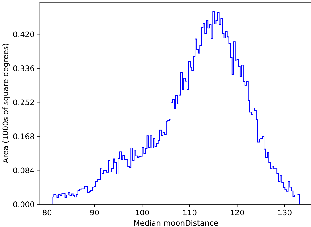
too_5_4v3.4_10yrs All sky r band: Median moonDistance
