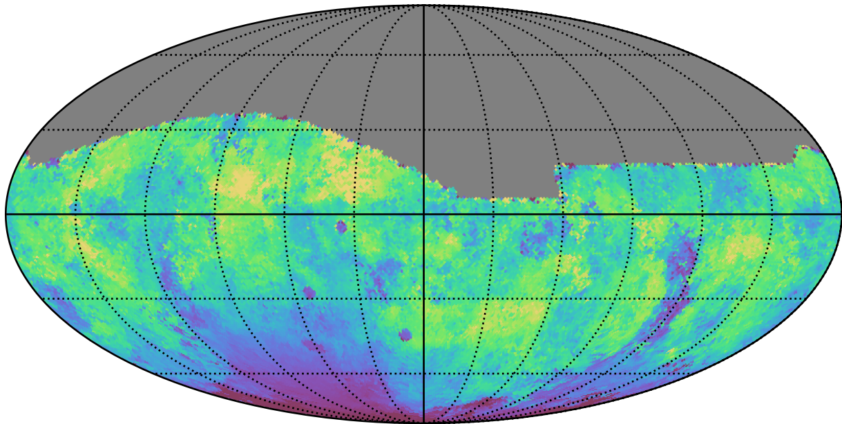
too_5_4v3.4_10yrs All sky g band: Median moonDistance
