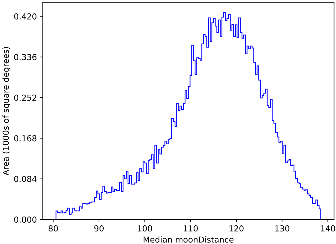
too_5_4v3.4_10yrs All sky g band: Median moonDistance
