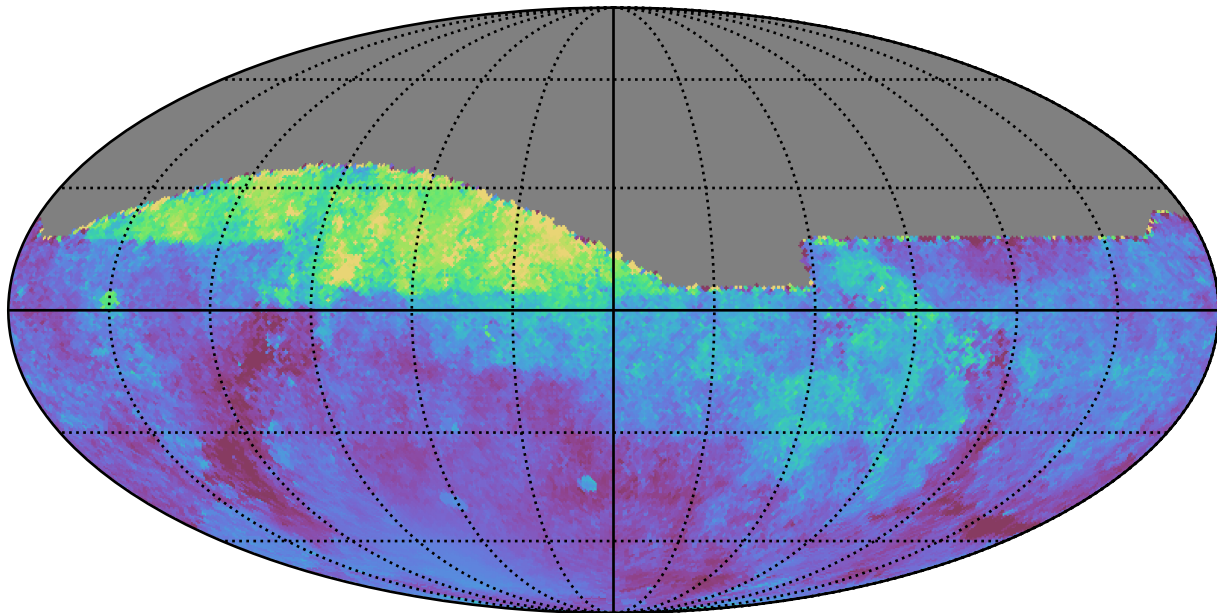
too_5_4v3.4_10yrs All sky all bands: Median moonDistance
