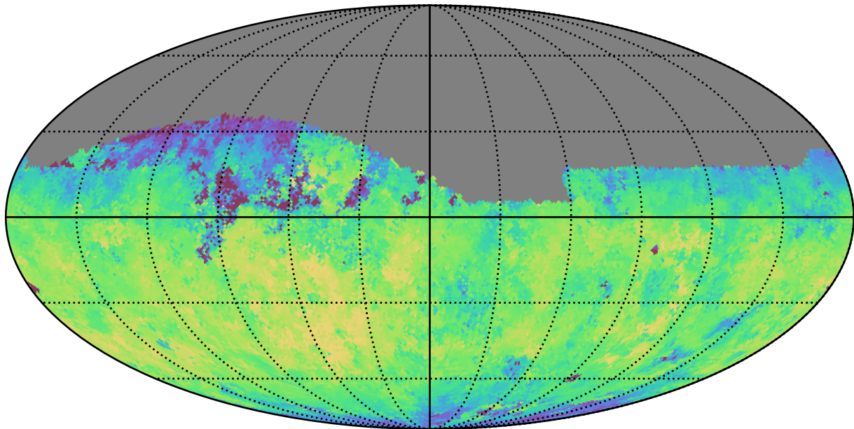
too_5_4v3.4_10yrs Yr 1 z band: Median fiveSigmaDepth
