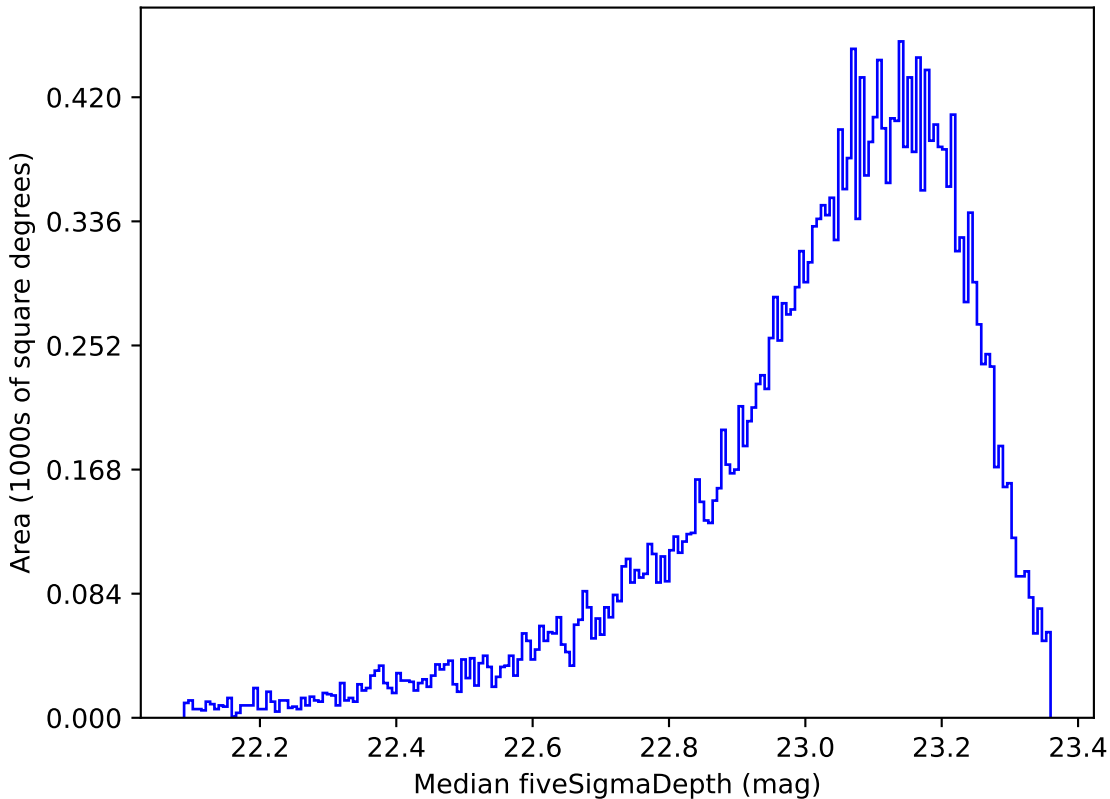
too_5_4v3.4_10yrs Yr 1 z band: Median fiveSigmaDepth
