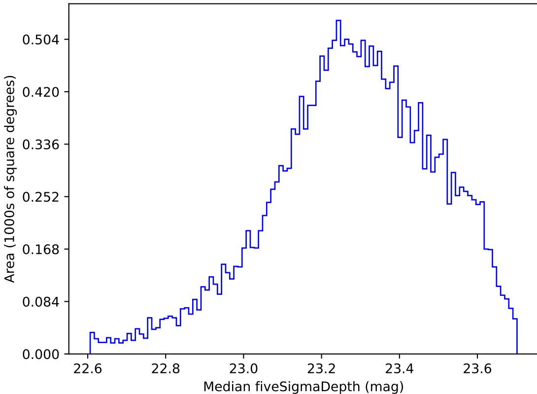
too_5_4v3.4_10yrs Yr 1 u band: Median fiveSigmaDepth
