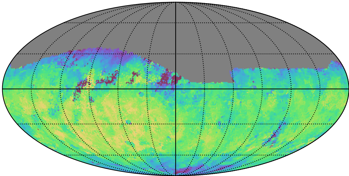
too_5_4v3.4_10yrs Yr 1 r band: Median fiveSigmaDepth
