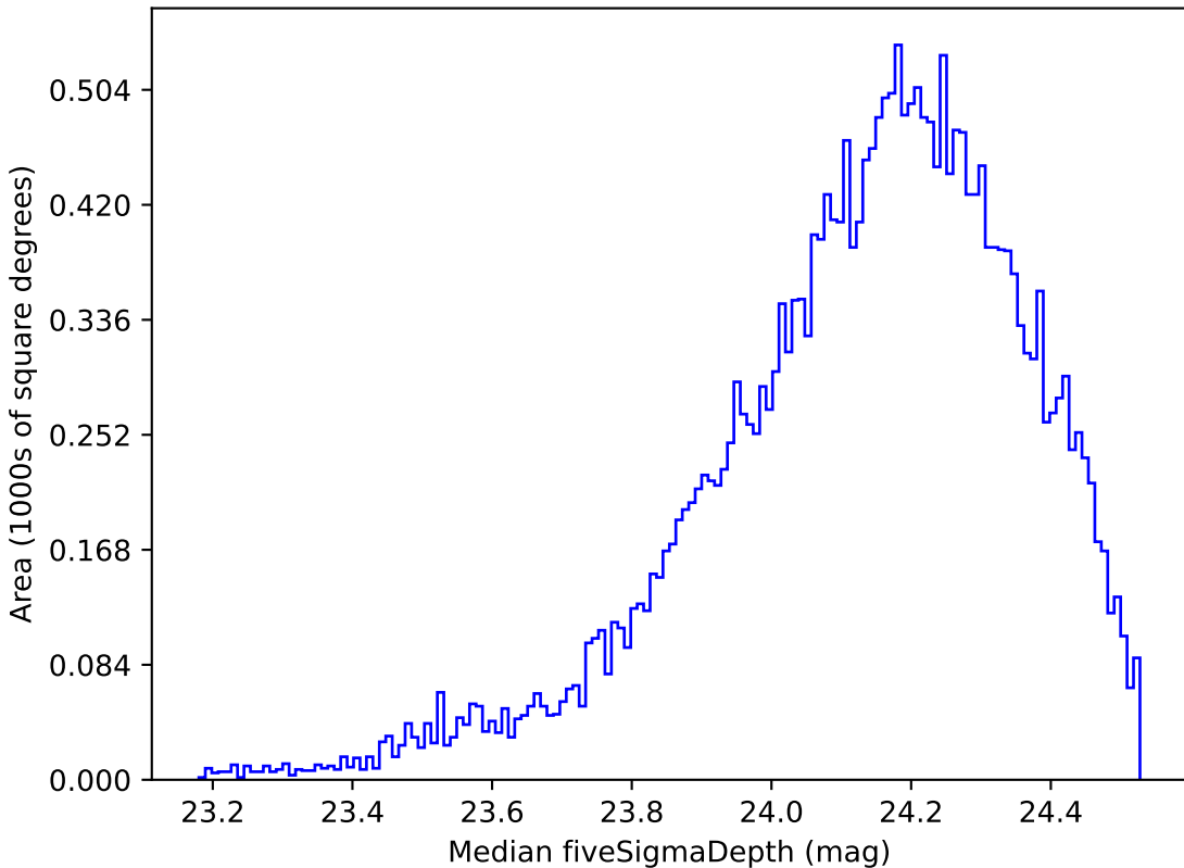
too_5_4v3.4_10yrs Yr 1 r band: Median fiveSigmaDepth
