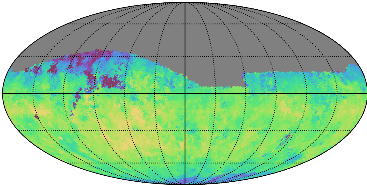
too_5_4v3.4_10yrs Yr 1 i band: Median fiveSigmaDepth
