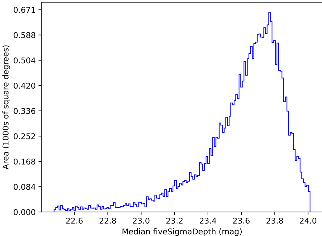
too_5_4v3.4_10yrs Yr 1 i band: Median fiveSigmaDepth
