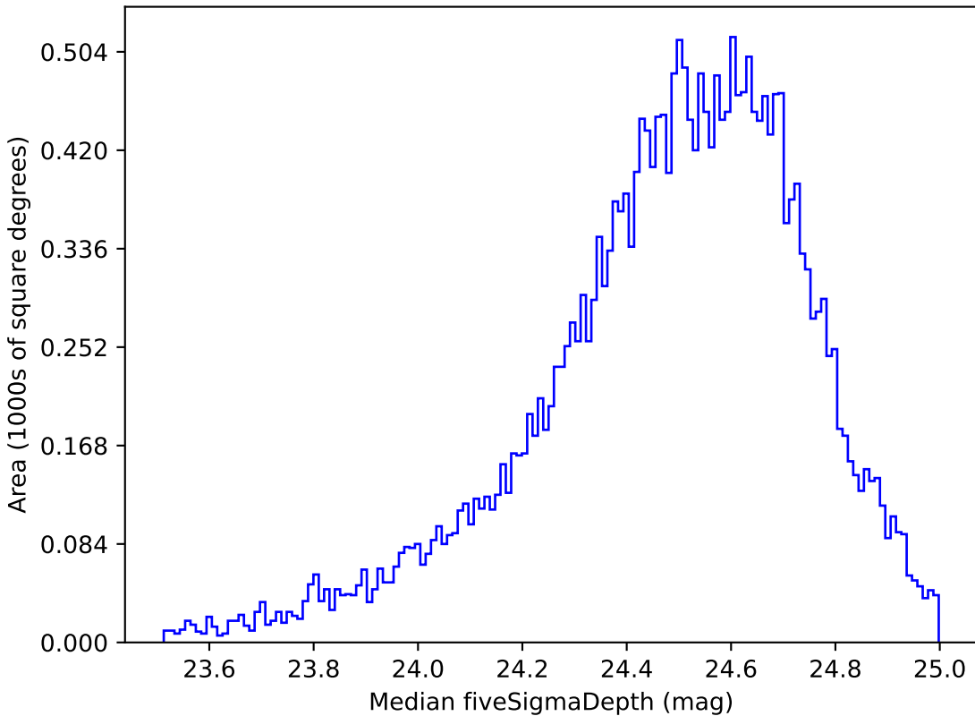
too_5_4v3.4_10yrs Yr 1 g band: Median fiveSigmaDepth
