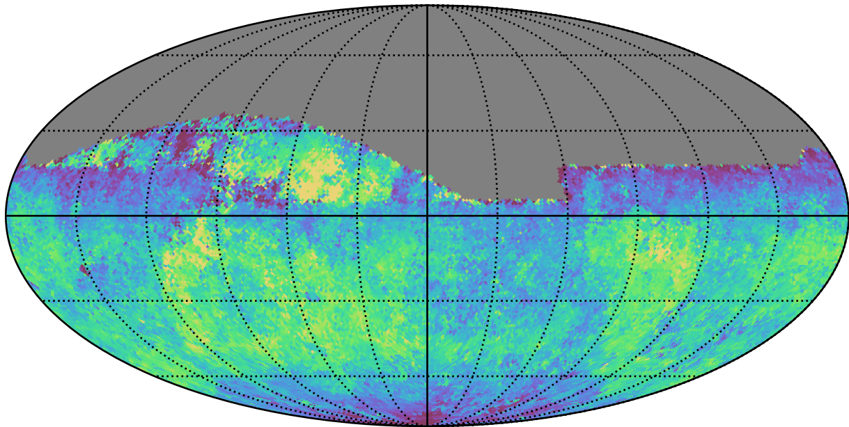
too_5_4v3.4_10yrs Yr 1 all bands: Median fiveSigmaDepth
