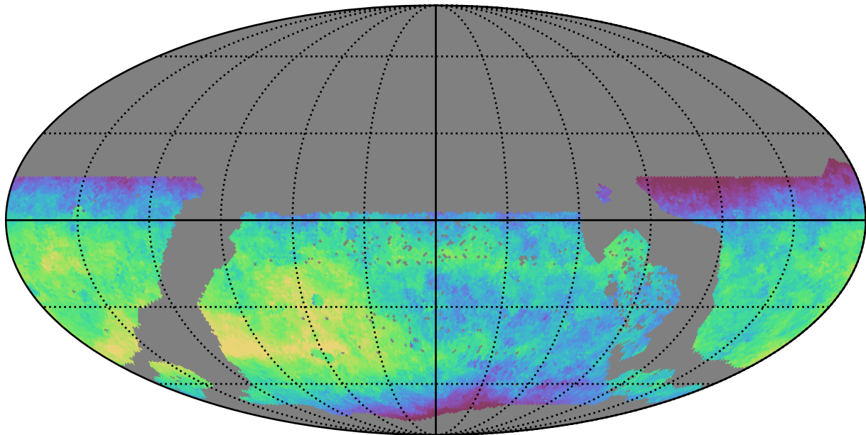
too_5_4v3.4_10yrs WFD z band: Median fiveSigmaDepth
