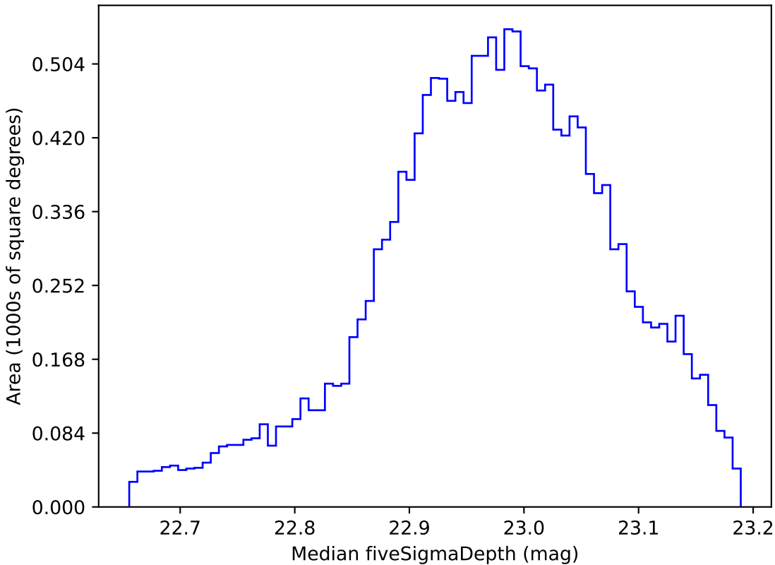
too_5_4v3.4_10yrs WFD z band: Median fiveSigmaDepth
