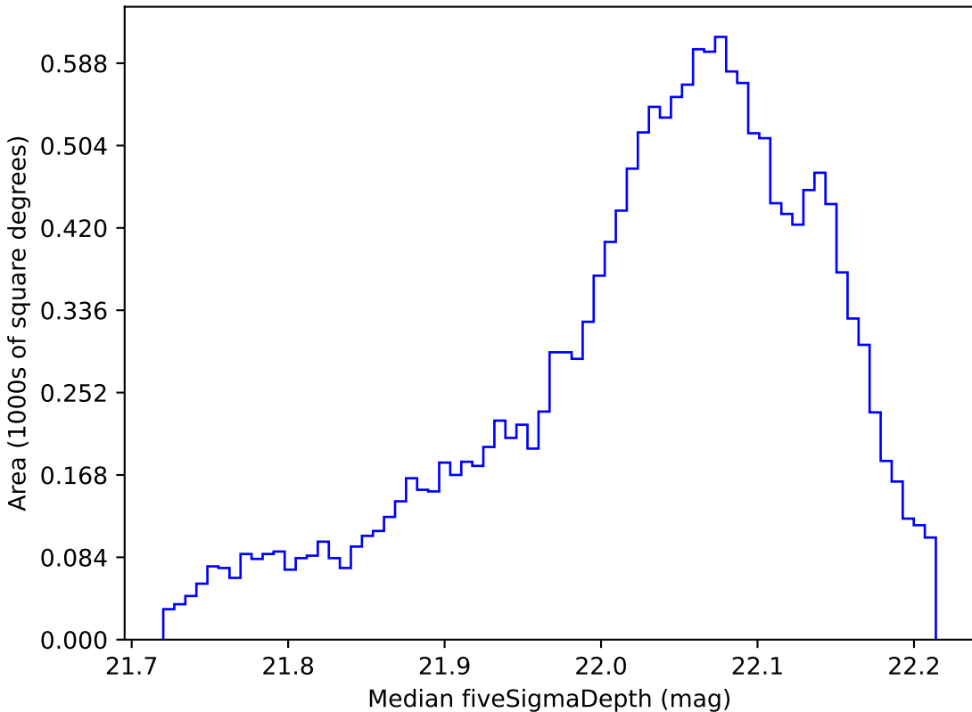
too_5_4v3.4_10yrs WFD y band: Median fiveSigmaDepth
