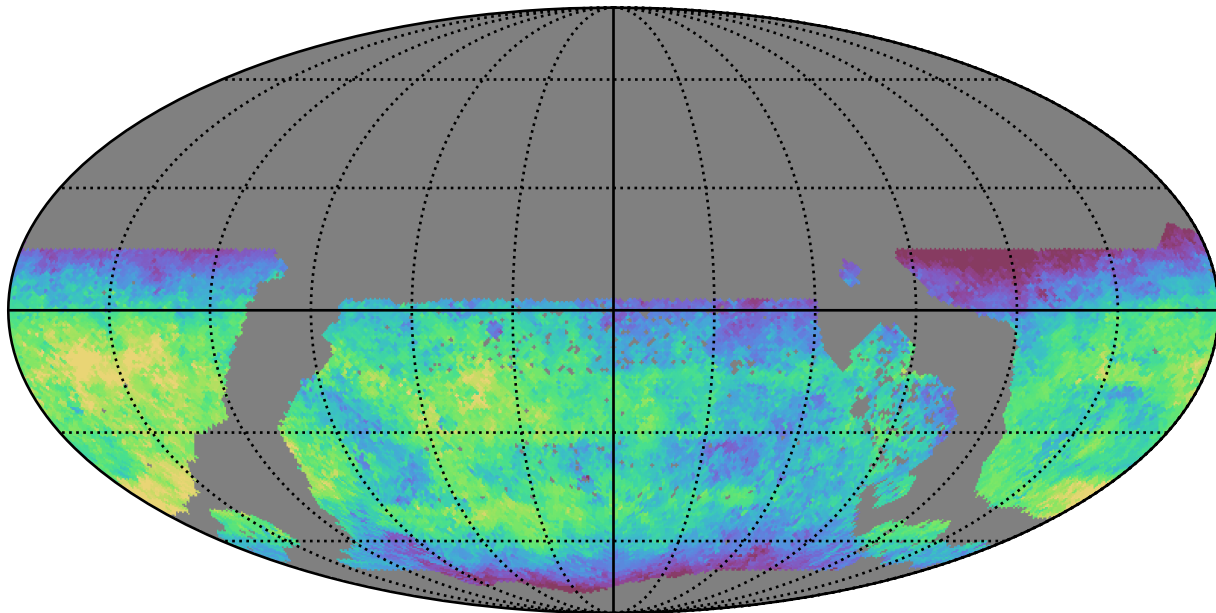
too_5_4v3.4_10yrs WFD u band: Median fiveSigmaDepth
