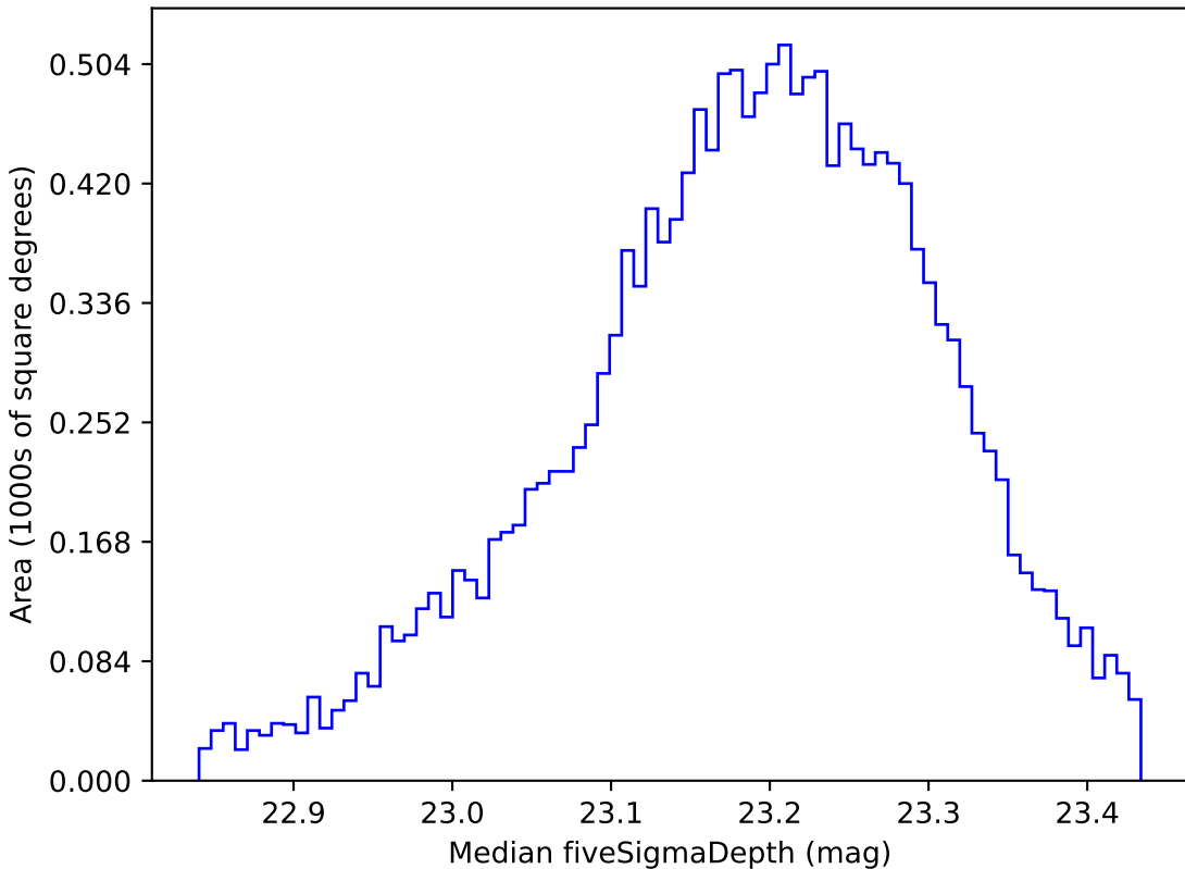
too_5_4v3.4_10yrs WFD u band: Median fiveSigmaDepth
