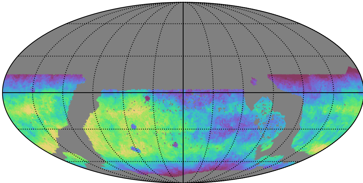
too_5_4v3.4_10yrs WFD r band: Median fiveSigmaDepth
