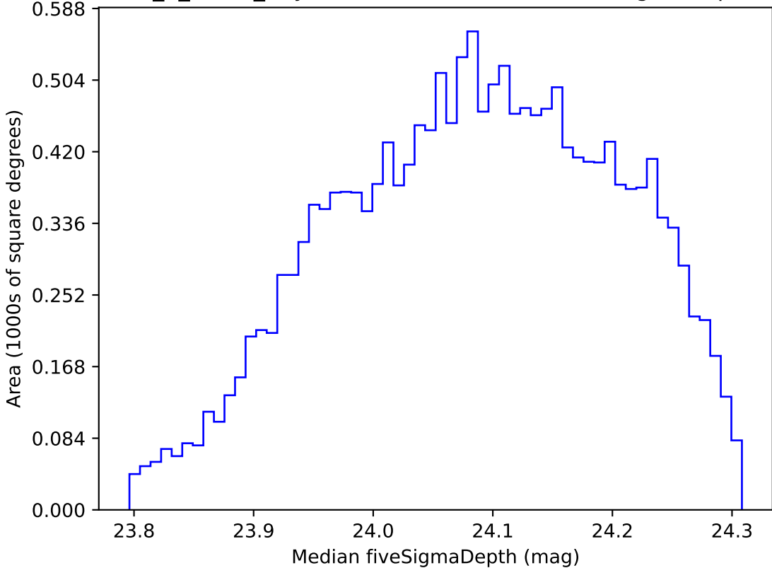
too_5_4v3.4_10yrs WFD r band: Median fiveSigmaDepth
